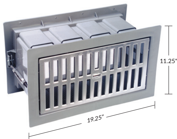
Vortex Manual BCV-80150 Dimensions: 19.25" W x 11.25" H Clear Vent Area (CVA) 31.4 – Screen included Each or 60/Pallet
