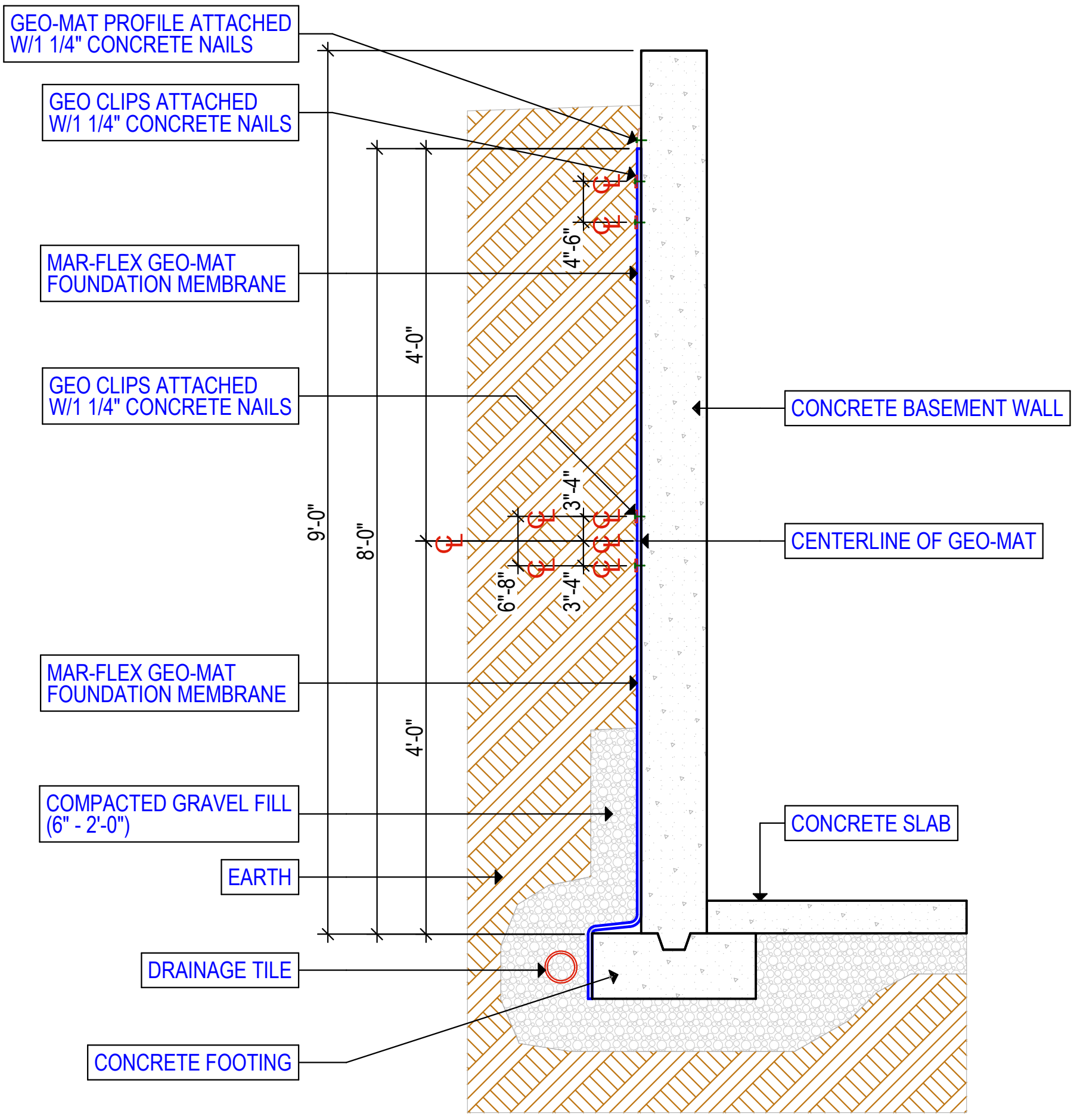
9'-0" WALL DETAIL (8'-0" HIGH GEO-MAT) GEO-MAT FOUNDATION WALL SECTION SCALE : 1/2" = 1'-0"
