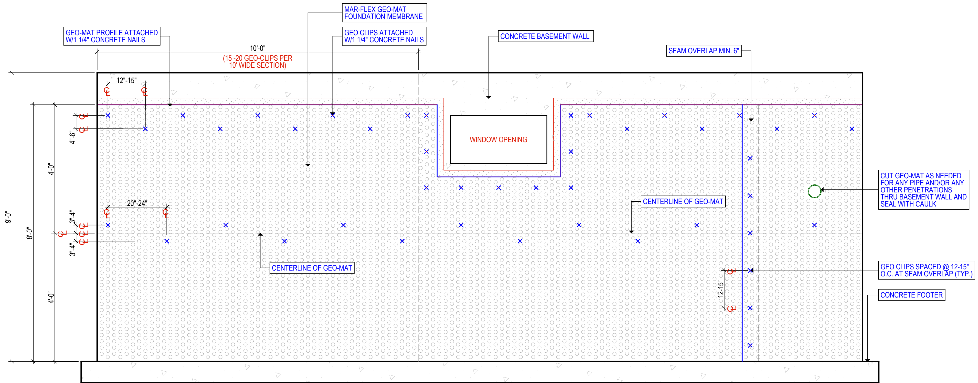
9'-0" WALL DETAIL (8'-0" HIGH GEO-MAT) GEO-MAT FOUNDATION WALL SECTION SCALE : 1/2" = 1'-0"
