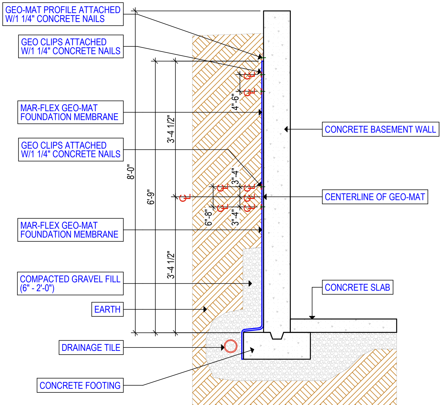
8'-0" WALL DETAIL (6'-9" HIGH GEO-MAT) GEO-MAT FOUNDATION WALL SECTION SCALE : 1/2" = 1'-0"
