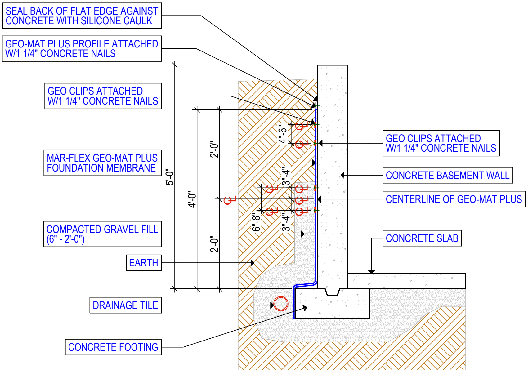
5'-0" WALL DETAIL (4'-0" HIGH GEO-MAT PLUS) GEO-MAT PLUS FOUNDATION WALL SECTION SCALE : 1/2" = 1'-0"
